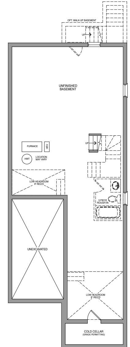
Basement ELEVATION C & F
