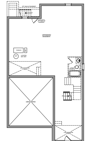
Basement ELEVATION C, F & T
