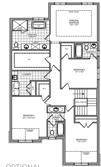
OPTIONAL Upper Floor ELEVATION F WITH 4 BEDROOMS
