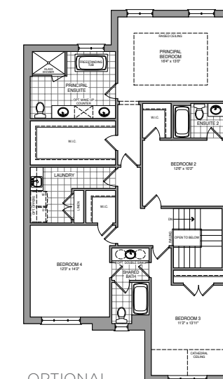
OPTIONAL Upper Floor ELEVATION T WITH 4 BEDROOMS
