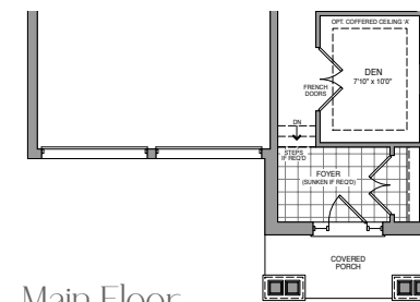
Main Floor ELEVATION T
