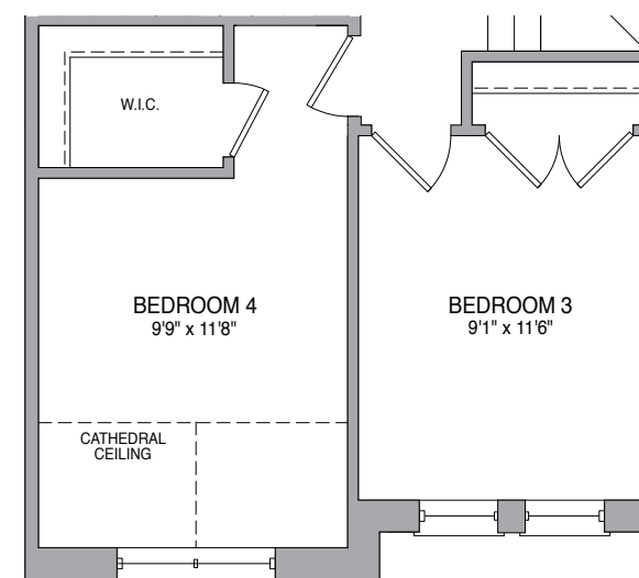
OPTIONAL Upper Floor ELEVATION F WITH 4 BEDROOMS
