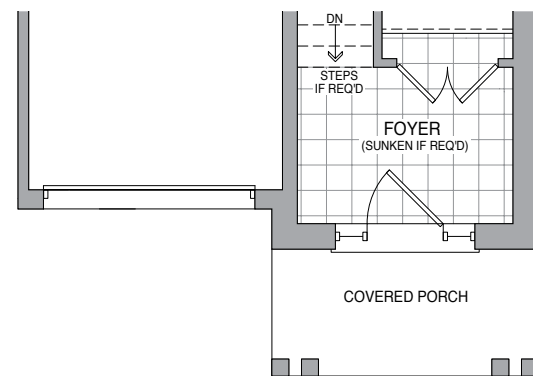
Main Floor ELEVATION F
