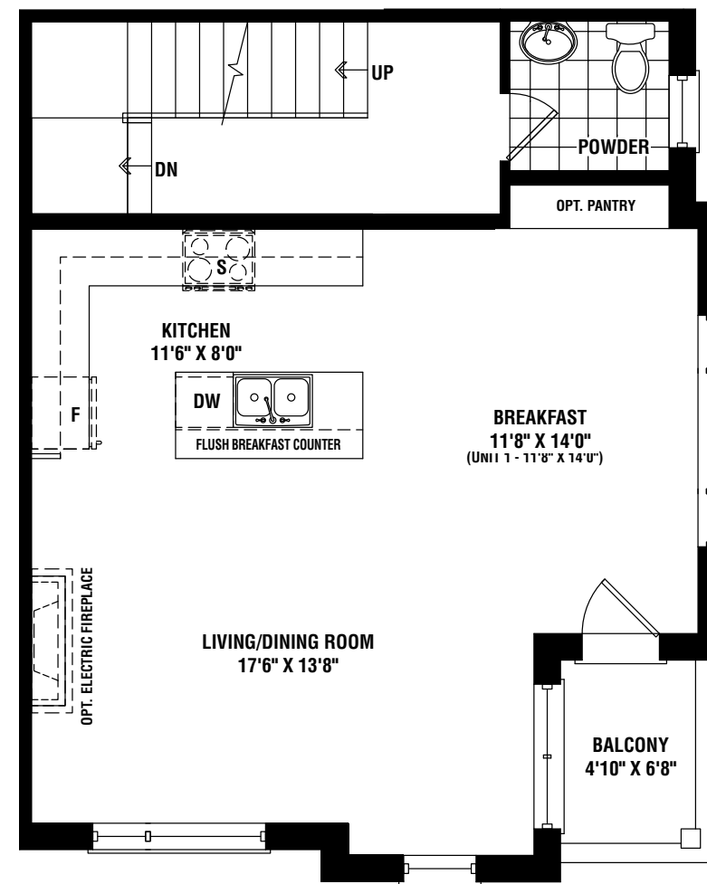
MAIN FLOOR ELEV. 'C1'
