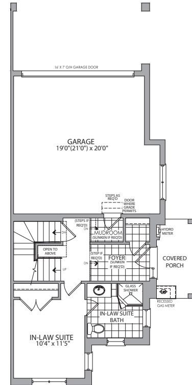
LOWER FLOOR OPT. IN-LAW SUITE ELEV. A
