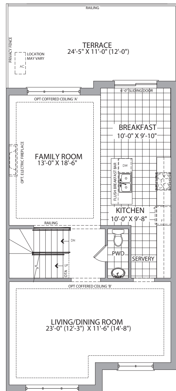
MAIN FLOOR ELEV. A
