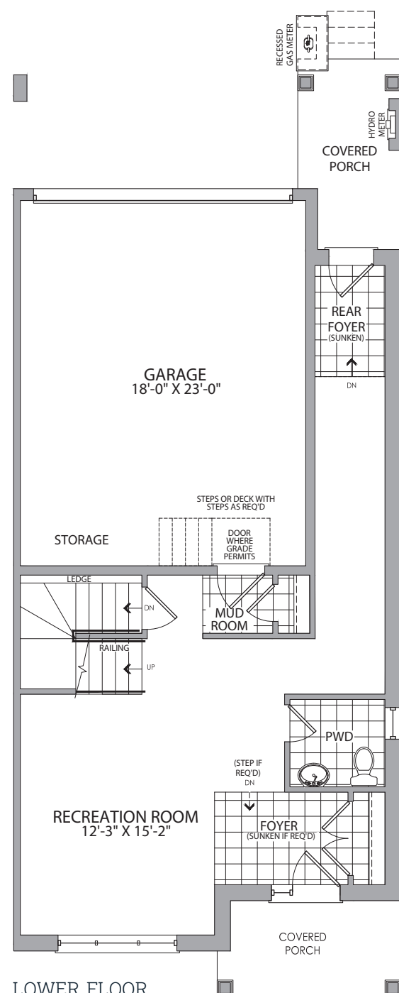
LOWER FLOOR ELEV. A
