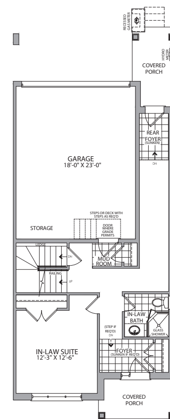
LOWER FLOOR OPT. IN-LAW SUITE ELEV. A
