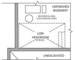
PARTIAL BASEMENT W/5 BEDROOM
