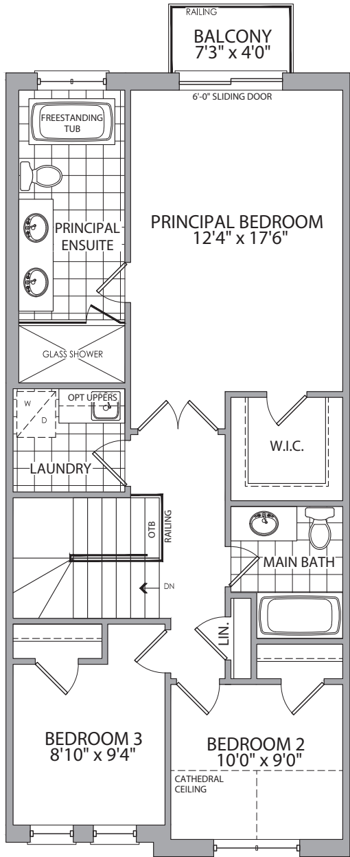
UPPER FLOOR ELEV. A1
