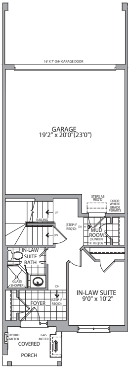
LOWER FLOOR OPT. IN-LAW SUITE ELEV. A1
