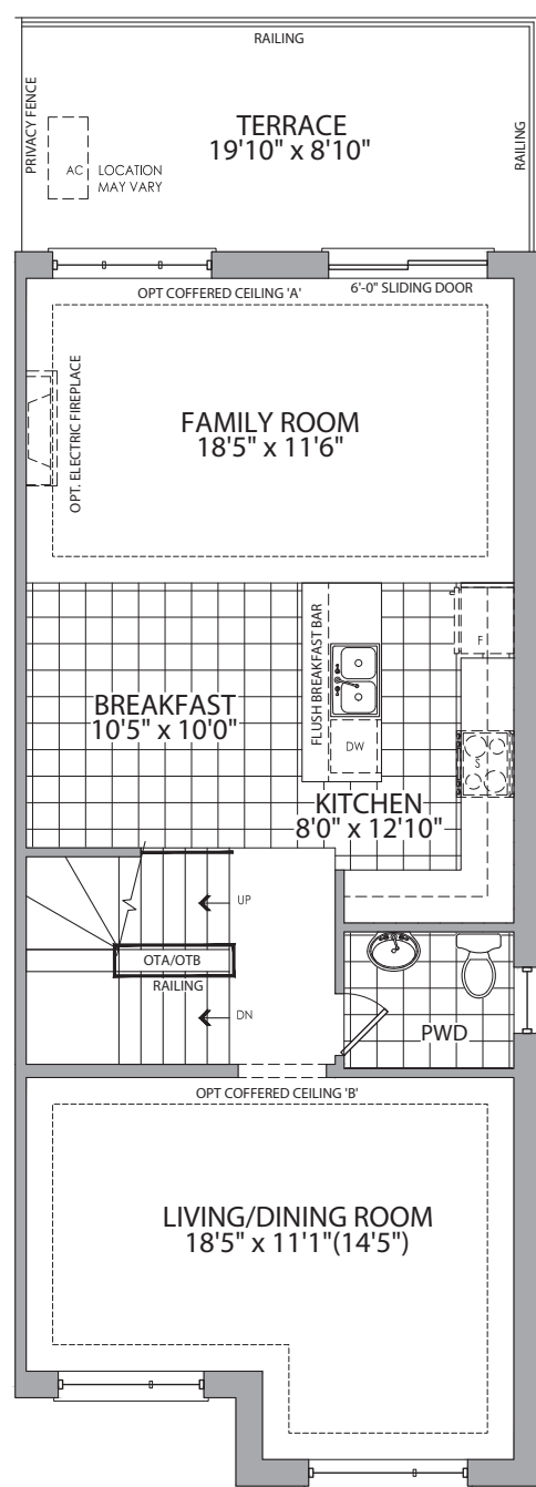
MAIN FLOOR ELEV. C
