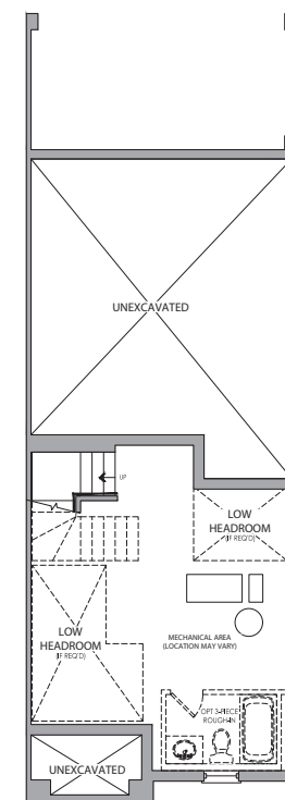
BASEMENT ELEV. C
