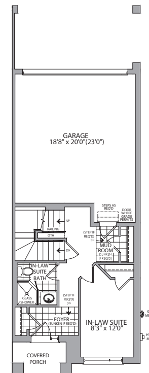
LOWER FLOOR OPT. IN-LAW SUITE ELEV. C
