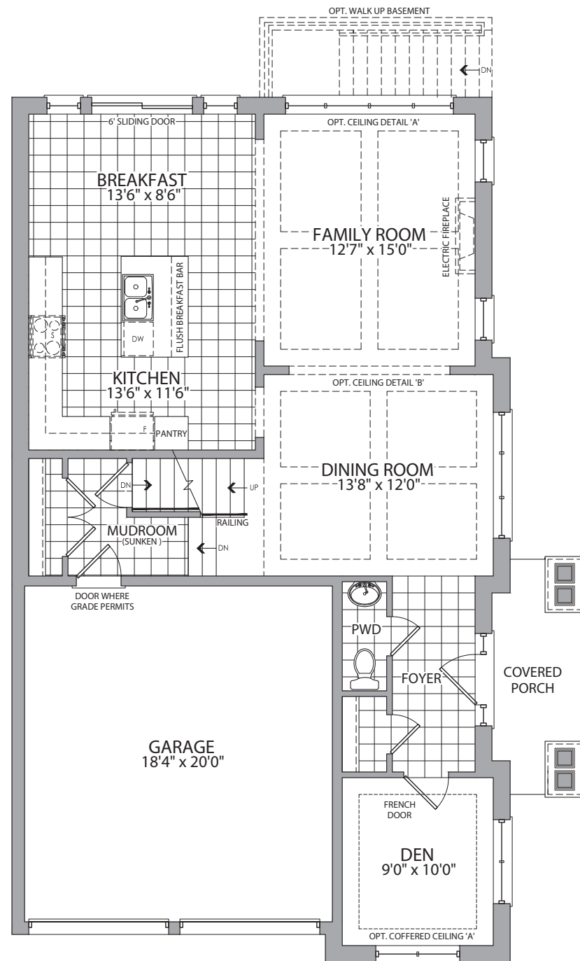
MAIN FLOOR ELEV. B
