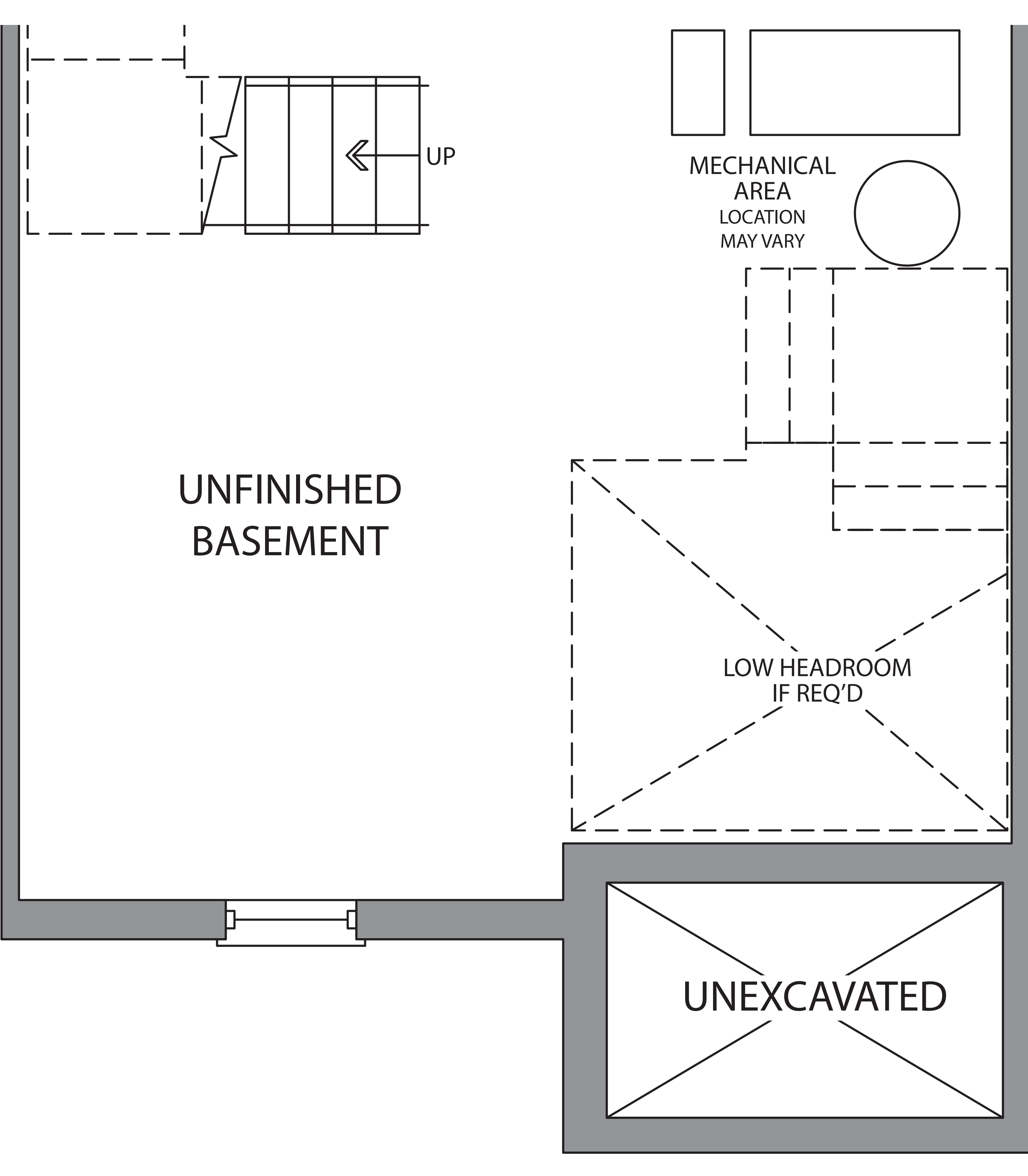
BASEMENT ELEV. F
