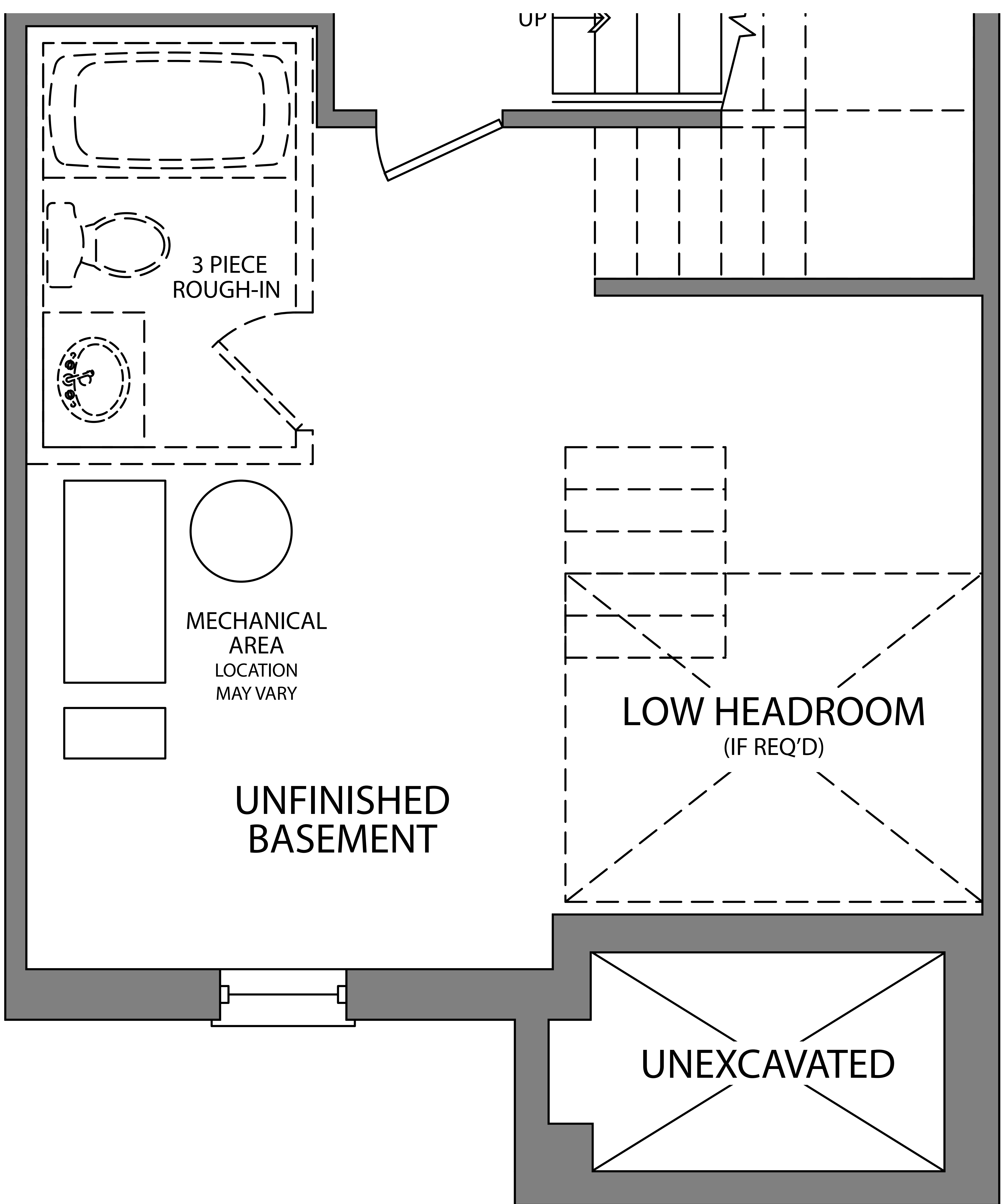
BASEMENT ELEV. C
