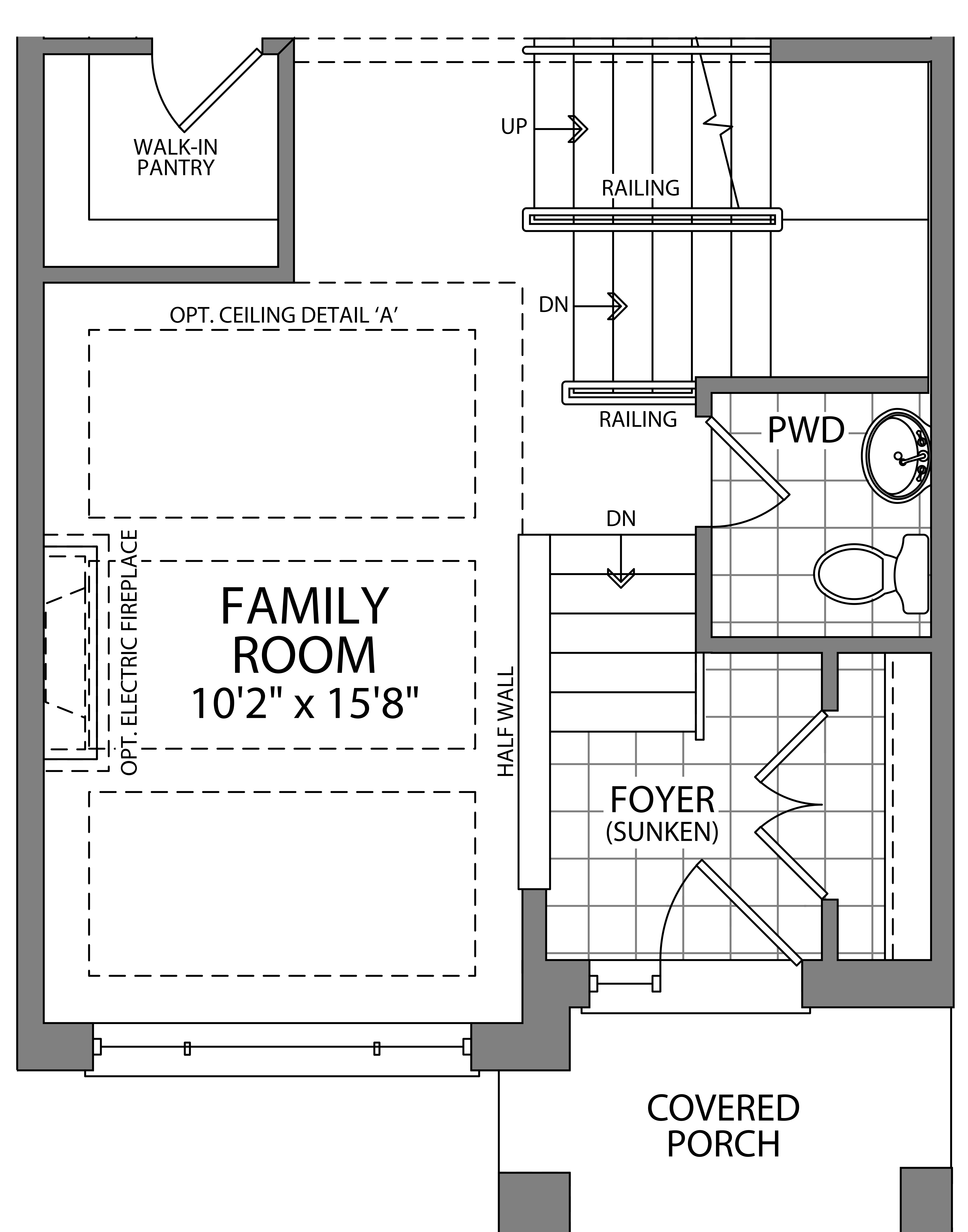
MAIN FLOOR ELEV. C
