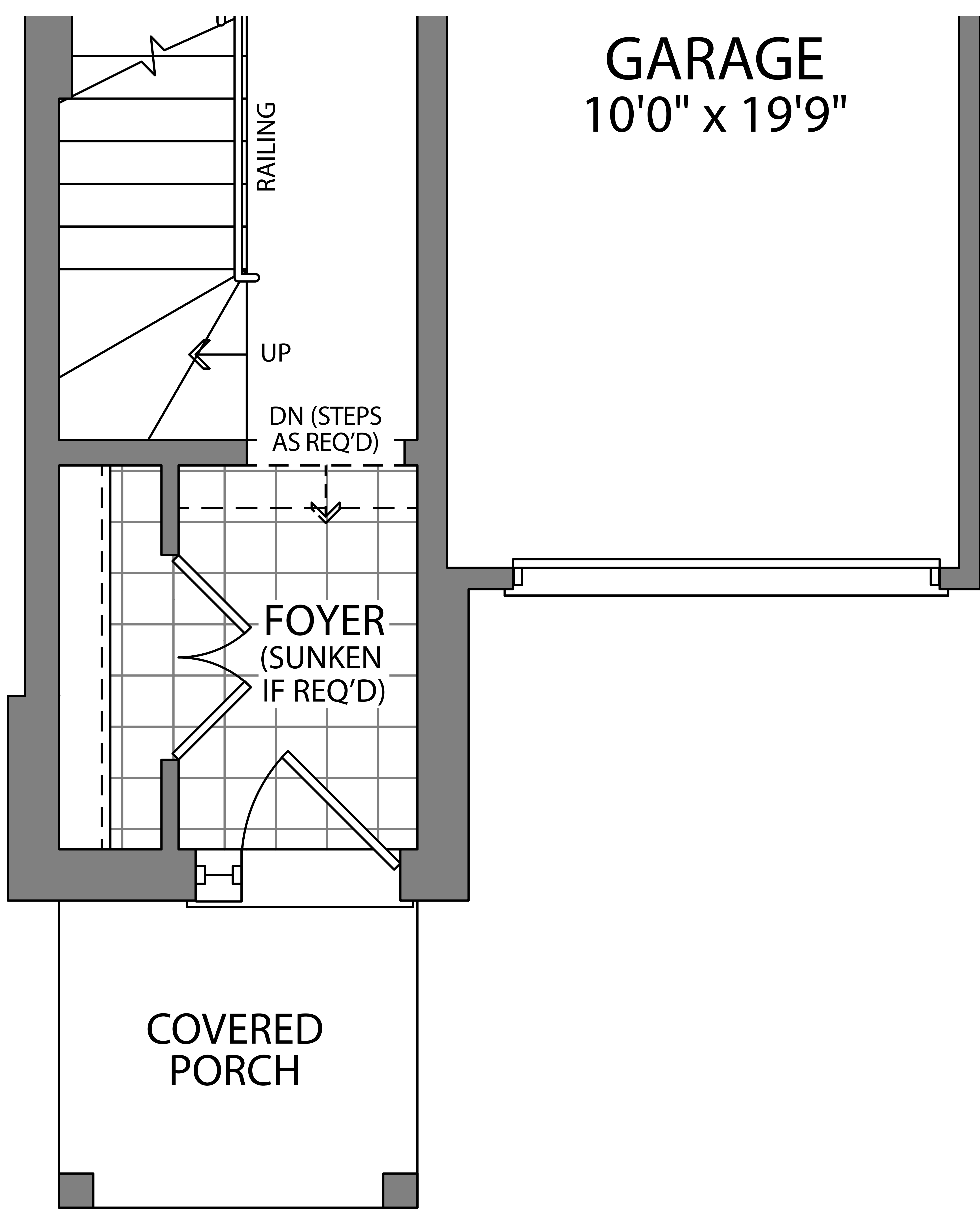
MAIN FLOOR ELEV. F
