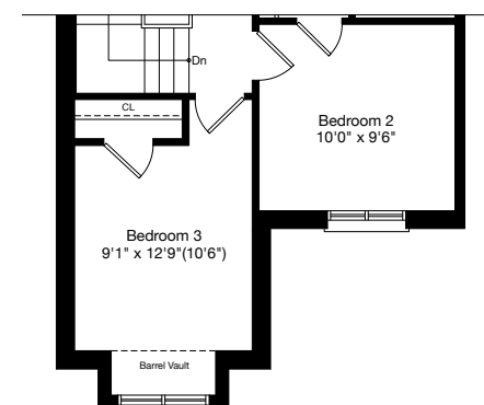
PARTIAL SECOND FLOOR ELEV. B1
