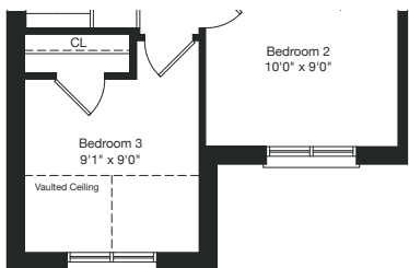
PARTIAL SECOND FLOOR ELEV. B1
