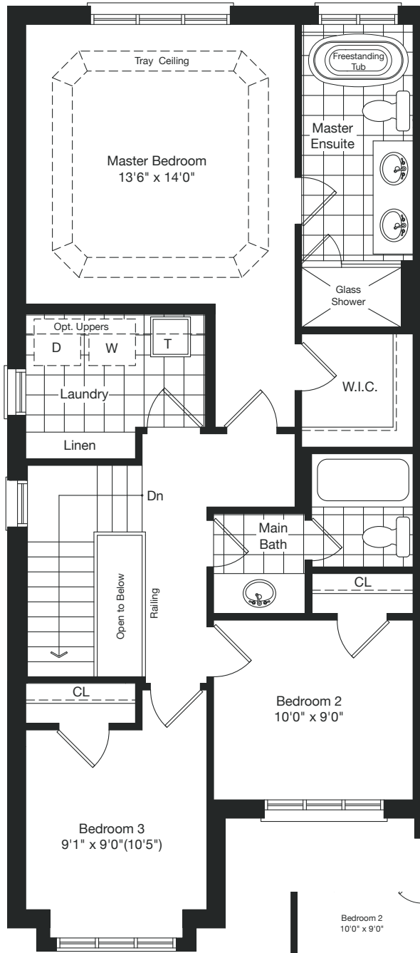
SECOND FLOOR ELEV. A1
