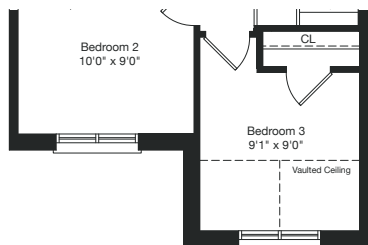
PARTIAL SECOND FLOOR ELEV. B2
