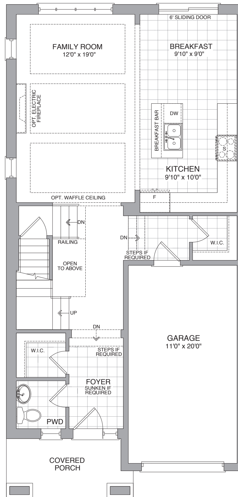
GROUND FLOOR ELEV C1 LEFT + RIGHT
