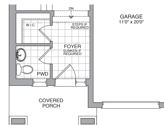
GROUND FLOOR ELEV C2 LEFT + RIGHT
