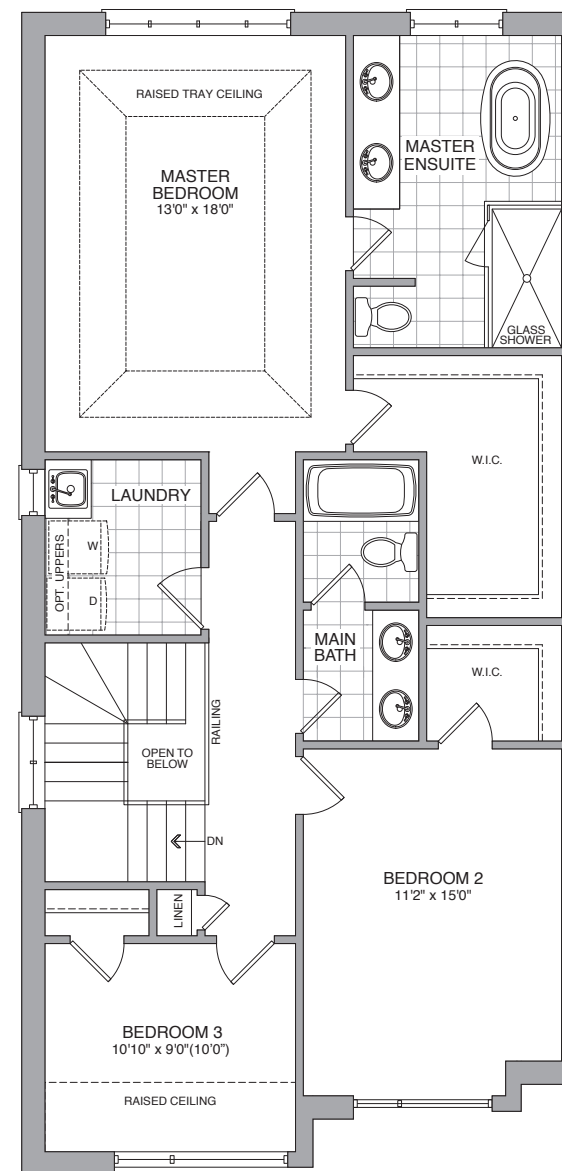
SECOND FLOOR ELEV C1 LEFT + RIGHT
