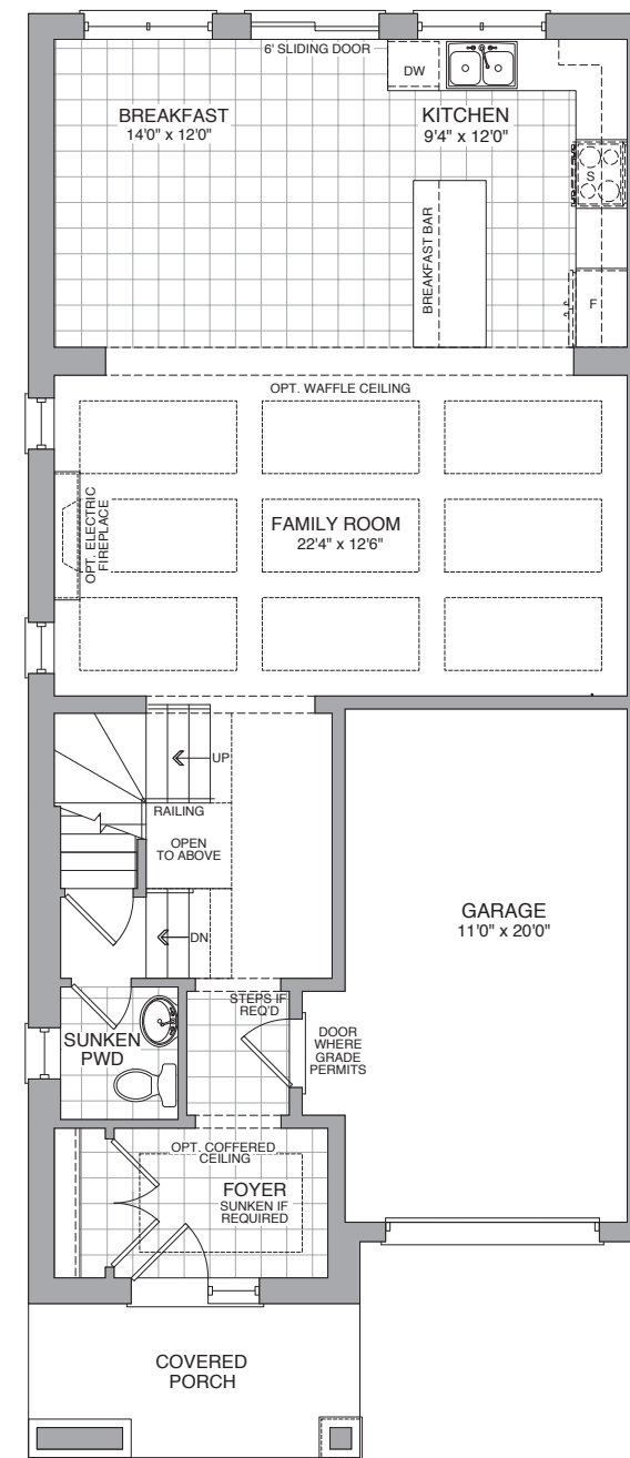
GROUND FLOOR ELEV C1 LEFT + RIGHT
