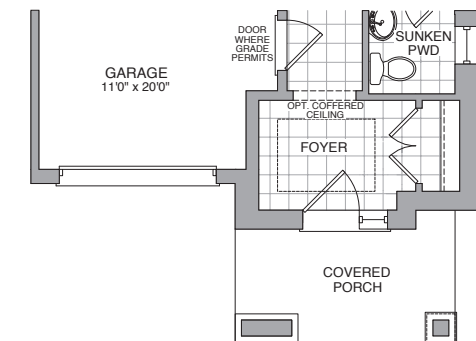
PARTIAL GROUND FLOOR ELEV C2 RIGHT
