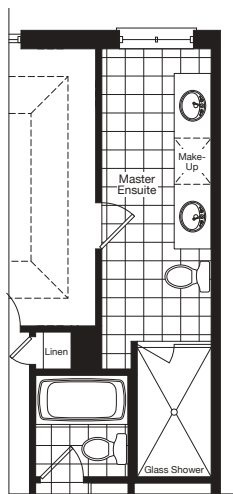
PARTIAL UPPER FLOOR OPT. MASTER ENSUITE ELEV. B-L & C-L
