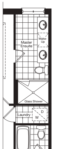
PARTIAL UPPER FLOOR OPT. 4 BEDROOM PLAN OPT. MASTER ENSUITE ELEV. B-L & C-L
