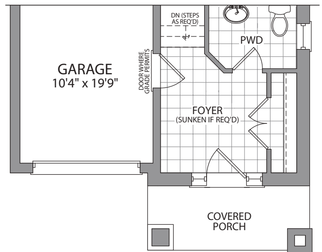
PARTIAL MAIN FLOOR ELEV. C
