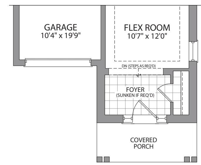
PARTIAL MAIN FLOOR ELEV. F
