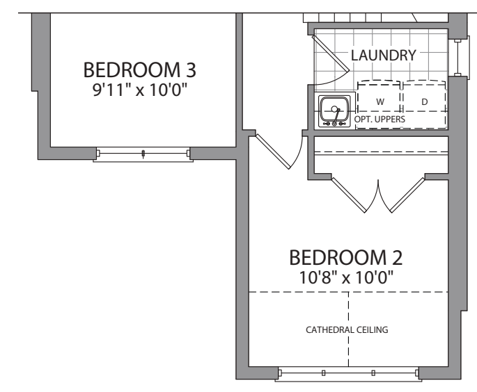
PARTIAL UPPER FLOOR ELEV. F
