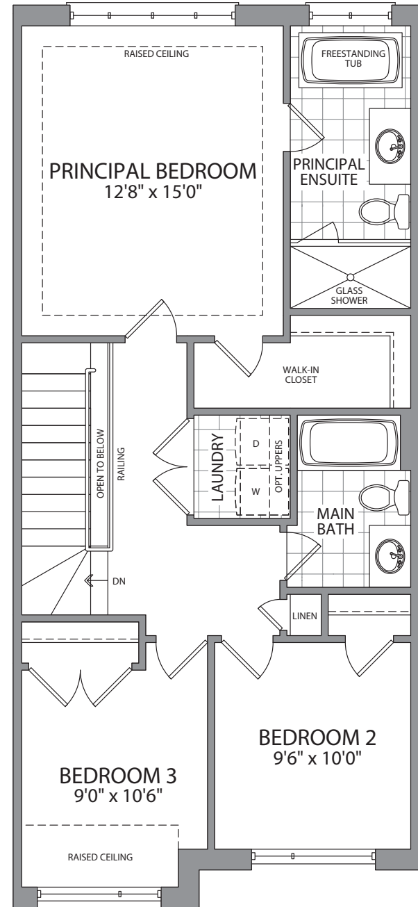
UPPER FLOOR ELEVATION C
