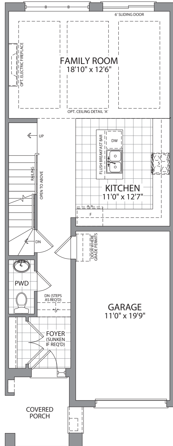
MAIN FLOOR ELEVATION C
