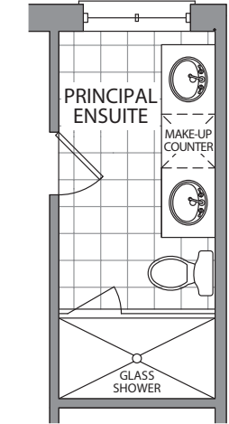
OPT. UPPER FLOOR PRINCIPAL ENSUITE ELEVATION F
