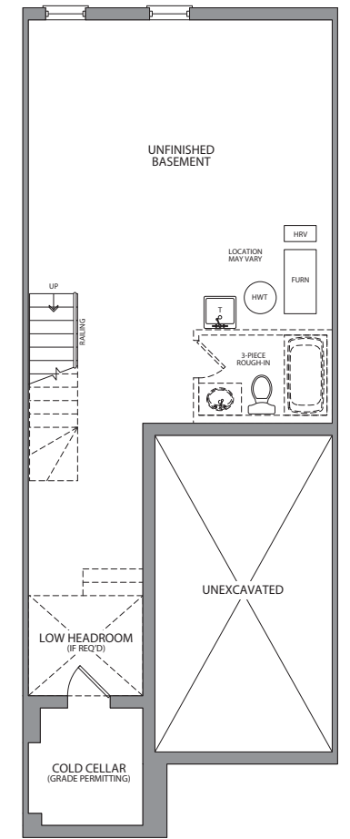
BASEMENT ELEVATION C + F
