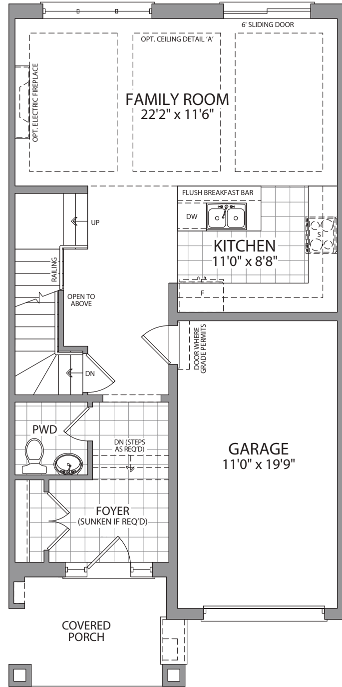
MAIN FLOOR ELEVATION C
