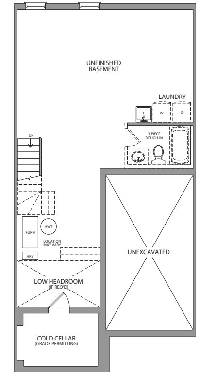
BASEMENT ELEVATION C + F
