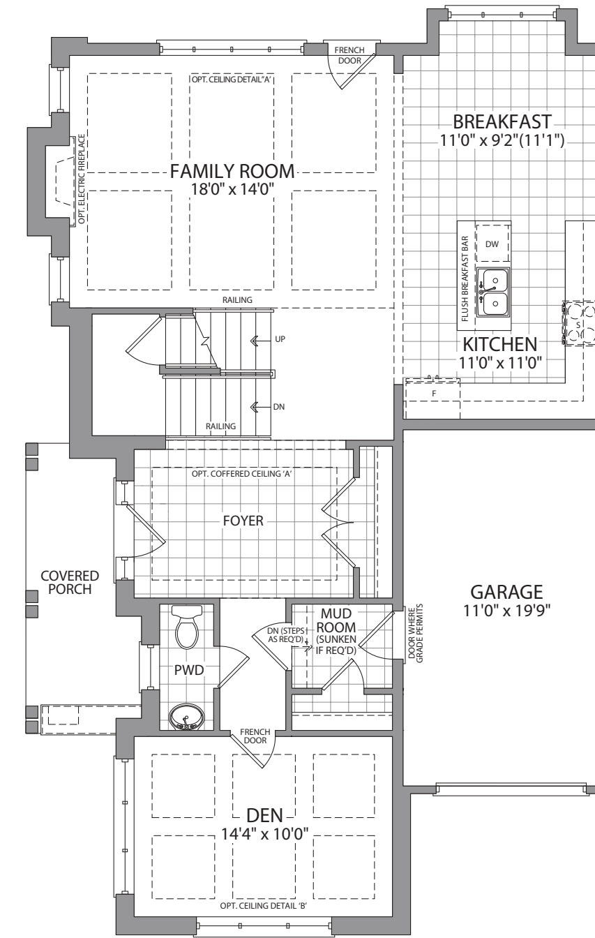
MAIN FLOOR ELEVATION F
