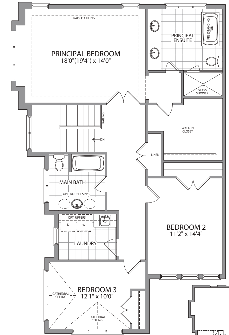
UPPER FLOOR ELEVATION F
