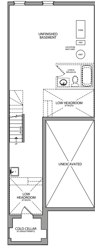
BASEMENT ELEV. C
