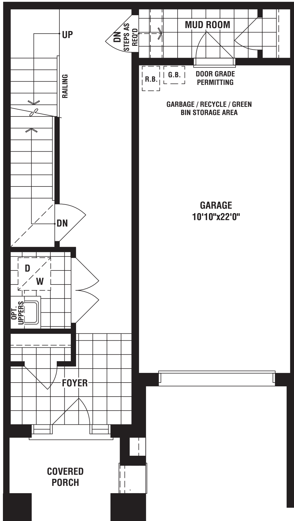
LOWER FLOOR ELEV. 'A'
