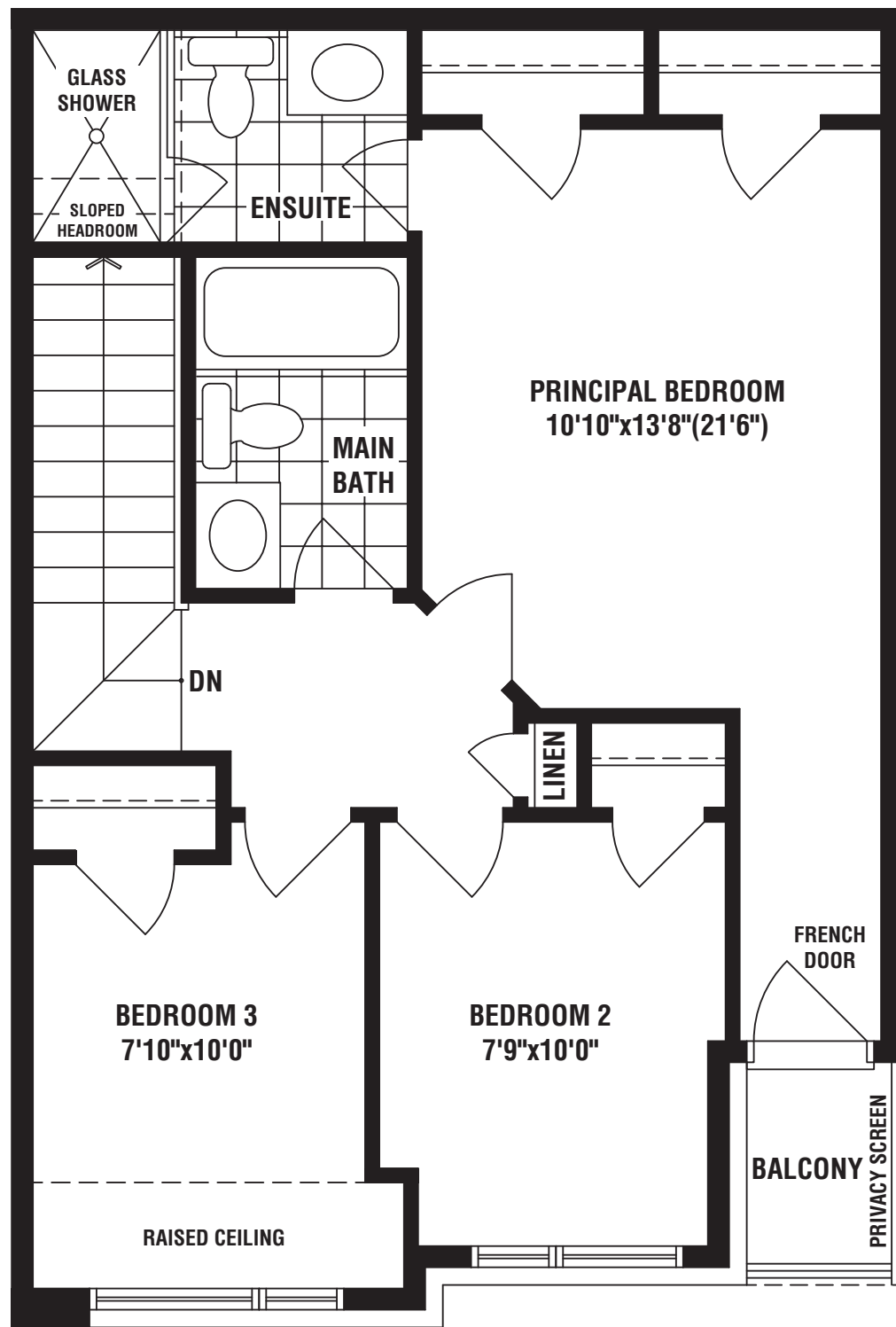
UPPER FLOOR ELEV. 'A'
