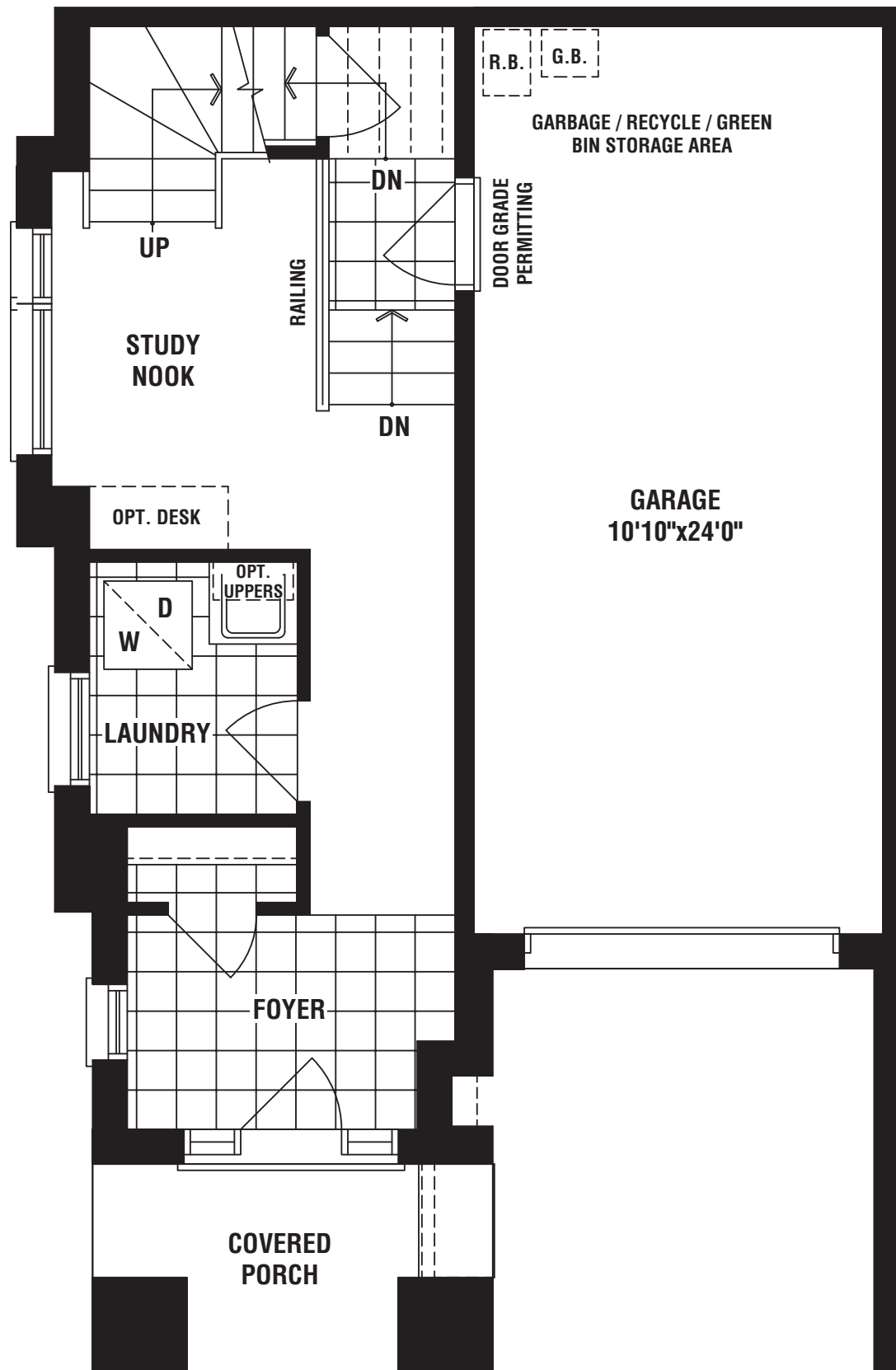
LOWER FLOOR ELEV. 'A'
