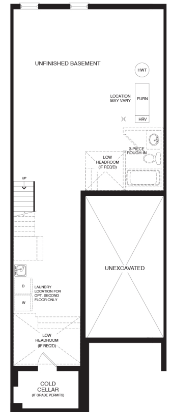
BASEMENT ELEV. C1 & C2
