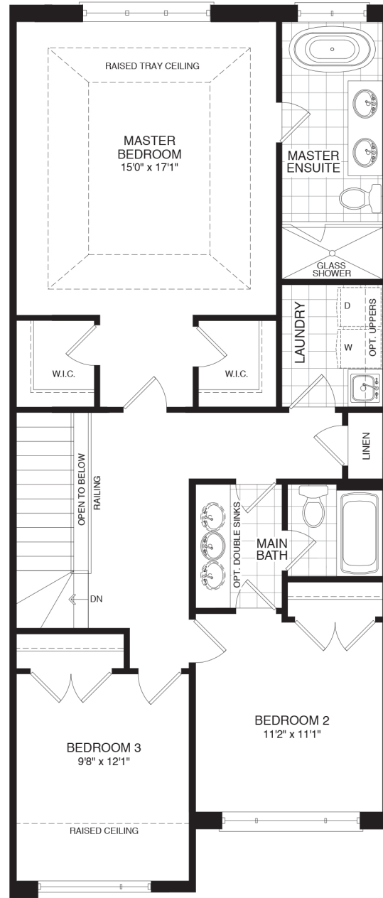
SECOND FLOOR ELEV. C1
