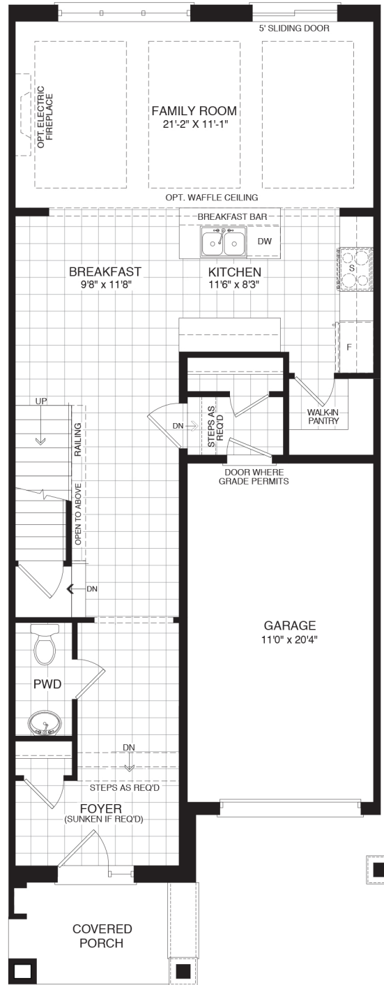
MAIN FLOOR ELEV. C1
