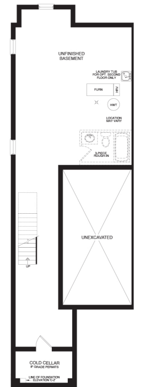
BASEMENT ELEV. C1 & C2
