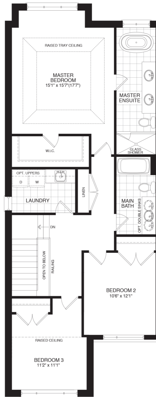
SECOND FLOOR ELEV. C1
