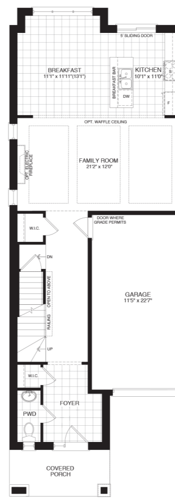
MAIN FLOOR ELEV. C2
