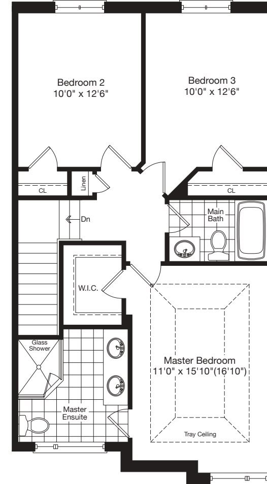
SECOND FLOOR ELEV. C1
